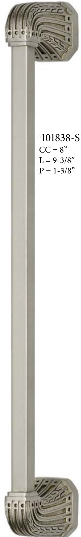
101836-MG CC = 6" L = 7-3/8" P = 1-3/8"
